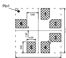
Solder area recommendation
