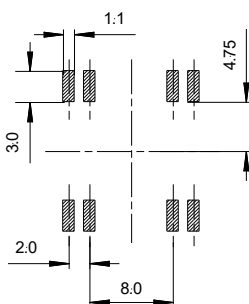
Solder area recommendation
