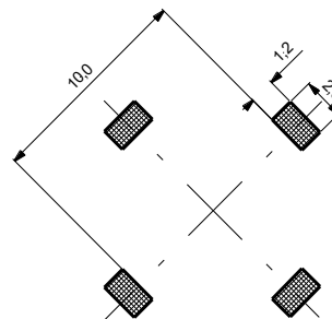
Solder area recommendation
