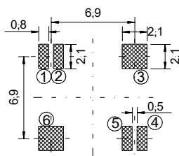
Solder area recommendation
