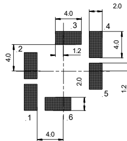
Solder area recommendation
